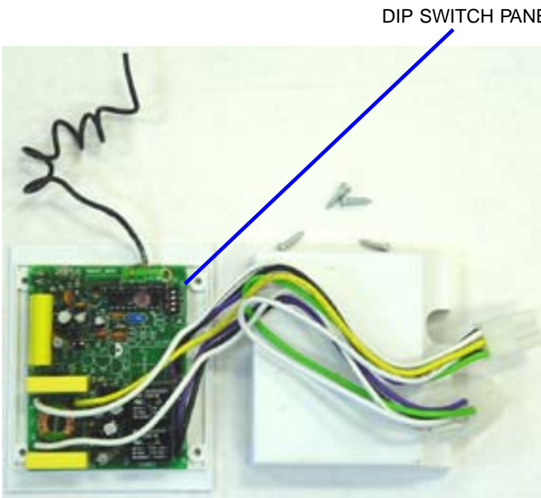
FIG. C RECEIVER
