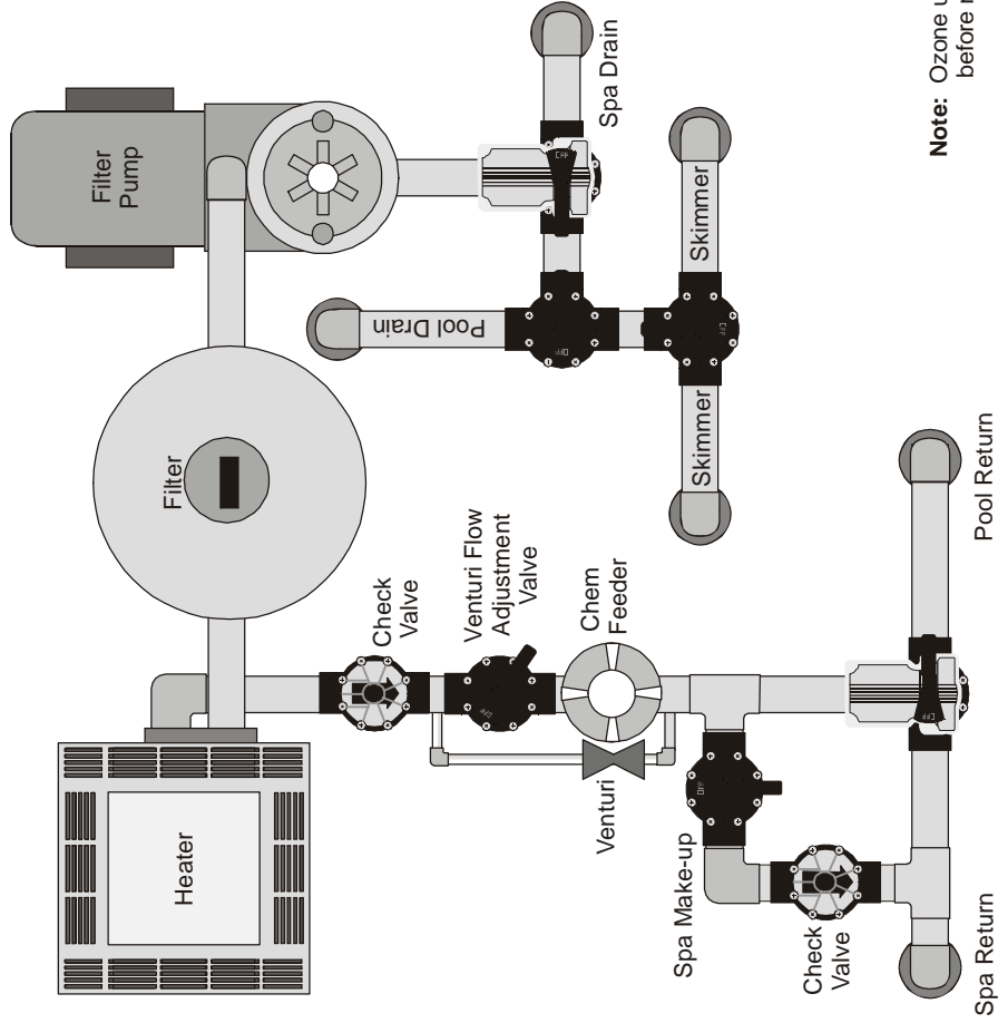
Inline Feeder / Bypass Venturi
