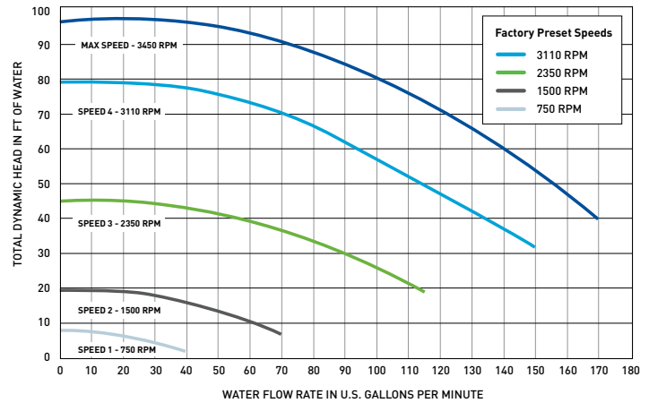
NOTE: The chart above demonstrates performance rates at factory preset speeds of 750 RPM, 1500 RPM, 2350 RPM and 3110 RPM.
