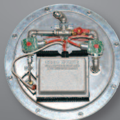
Burner Assembly
