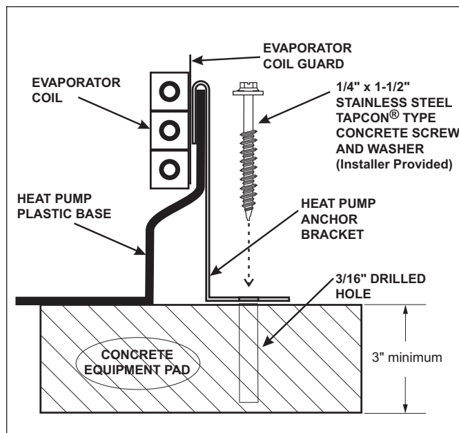
Figure 3. Anchor Clamp Installation
