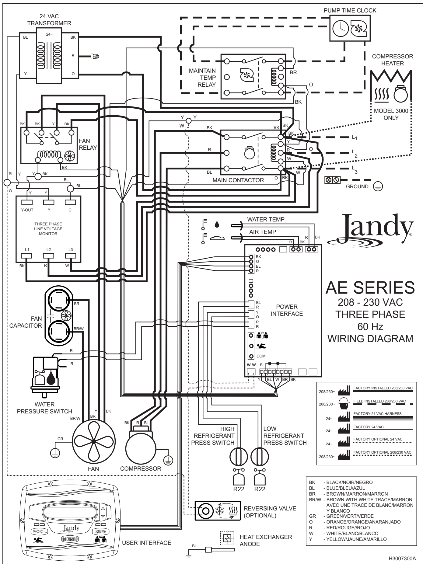
Figure 9. AE-Ti 3-Phase Electrical Supply Wiring Diagram
