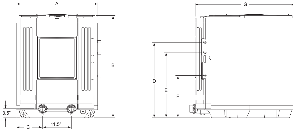
Figure 1. Jandy AE-Ti Heat Pumps Dimensions
