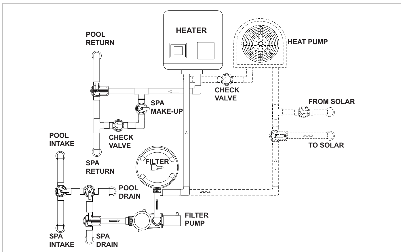
Figure 5. Plumbing For Heating System Combinations
