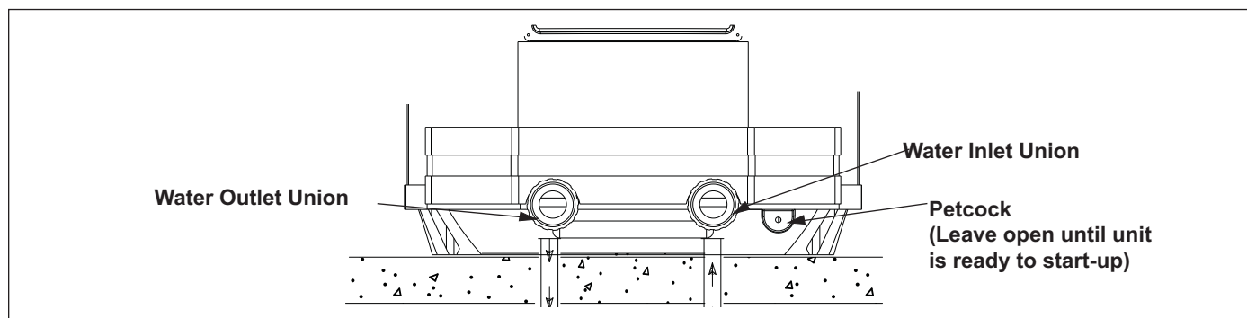
Figure 15. Winterizing the AE-Ti Heat Pump
