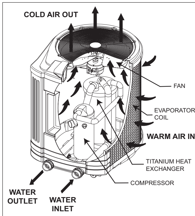
Figure 16. Heat Pump Operation Overview
