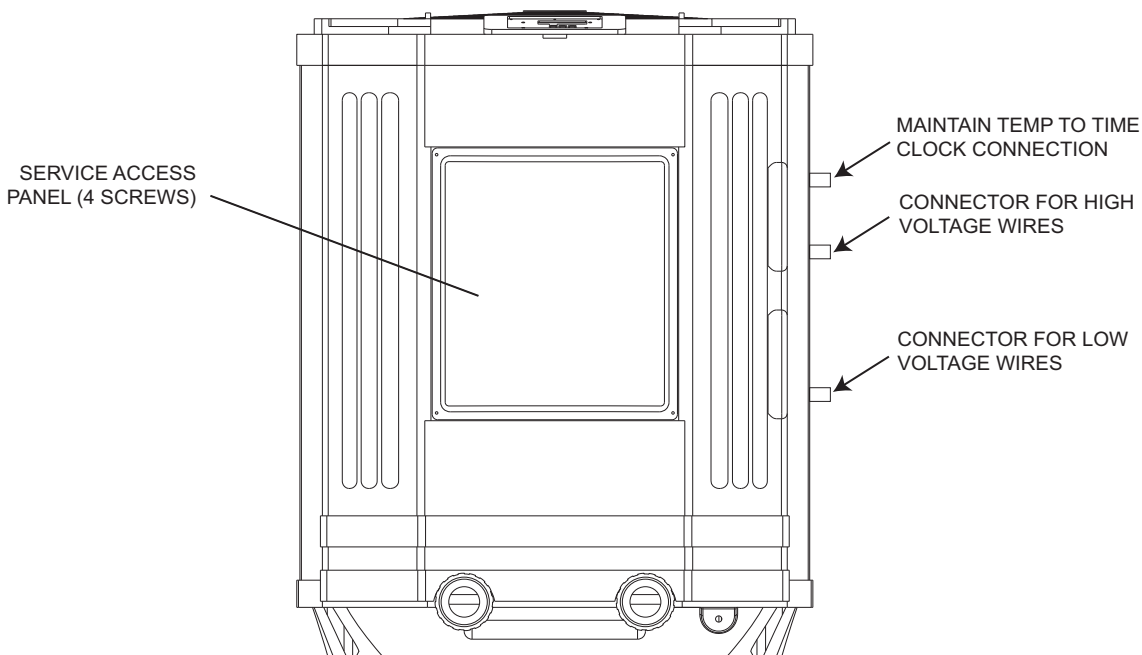
Figure 11. AE-Ti Heat Pump Front View
