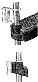
Diagram 2: Procedure for bushing installation
