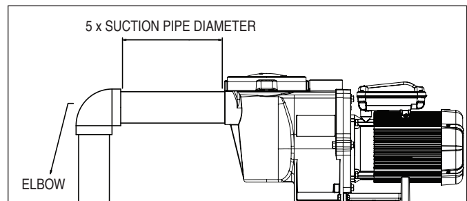
Recommended Piping
