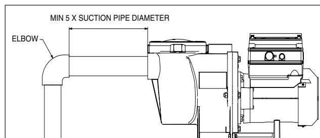
Figure 2: Recommended Piping
